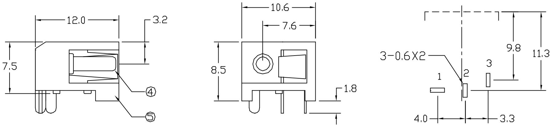
PCB LAYOUT (BOTTOM VIEW)
